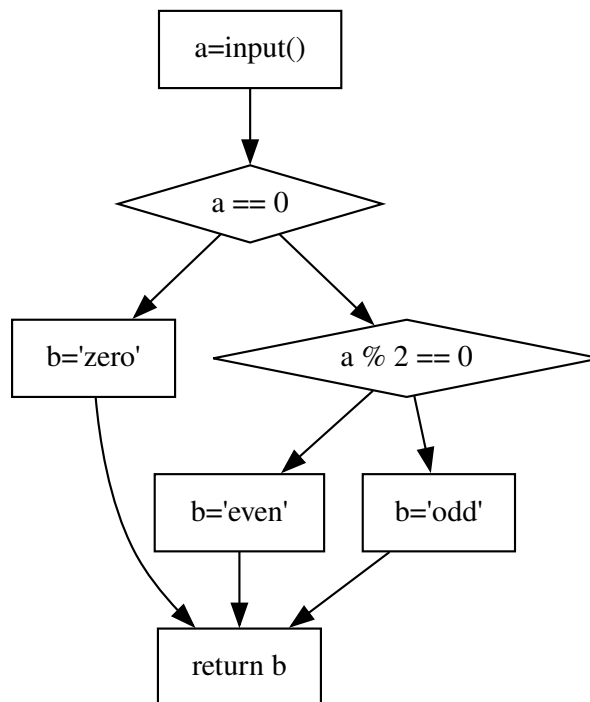
Figure 142: Flow diagram of the program we'll calculate the cyclomatic complexity of
